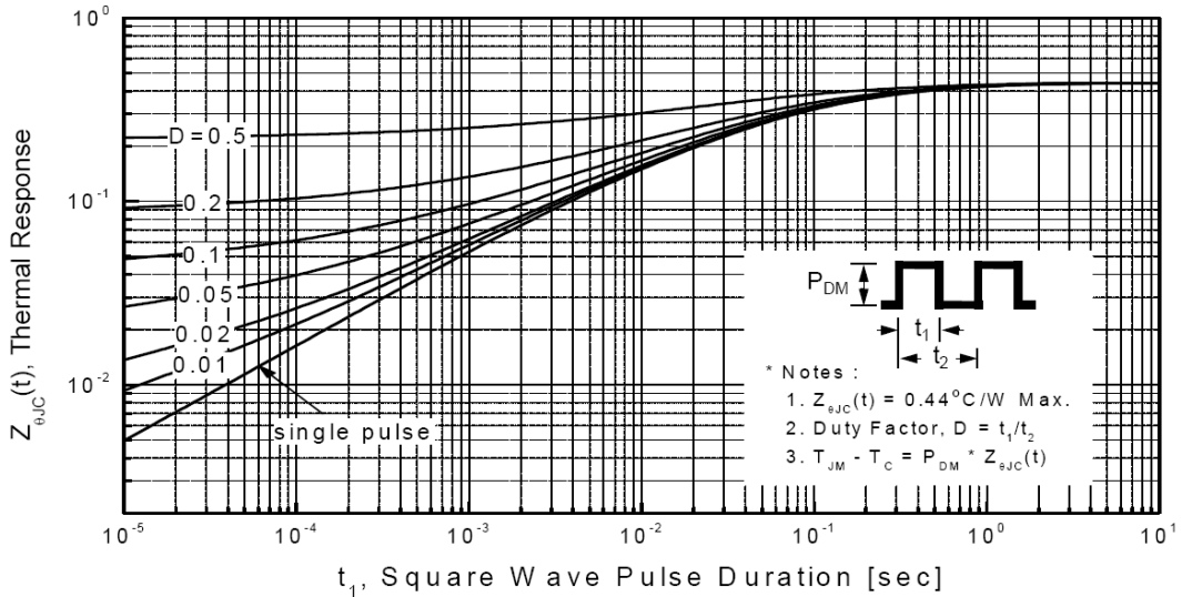
图10. 瞬态热响应曲线(TO-247) Fig. 10 Transient Thermal Response Curve (TO-247)
