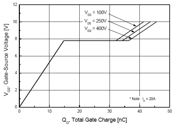
图6. 栅电荷特性曲线 Fig. 6 Gate Charge Characteristics
