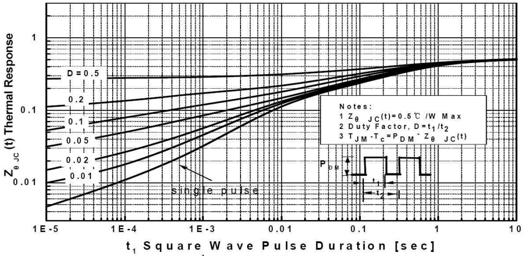
图9. 瞬态热响应曲线(TO-3PN) Fig. 9 Transient Thermal Response Curve (TO-3PN)
