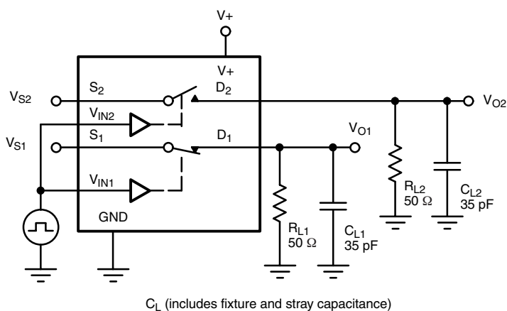
Figure 2. Break-Before-Make (DG2739)
