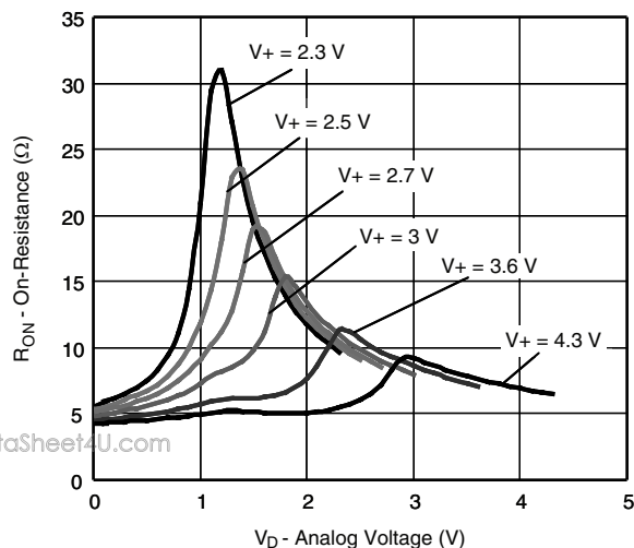
R ON vs. V D and Supply Voltage
