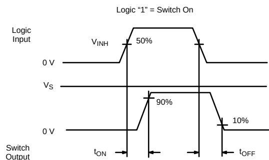
FIGURE 2. Switching Time
