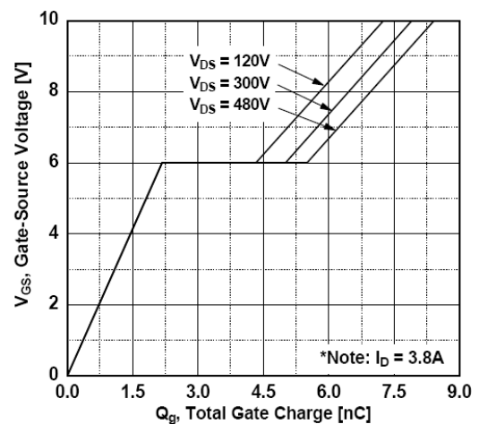
图6. 栅电荷特性曲线 Fig. 6 Gate Charge Characteristics
