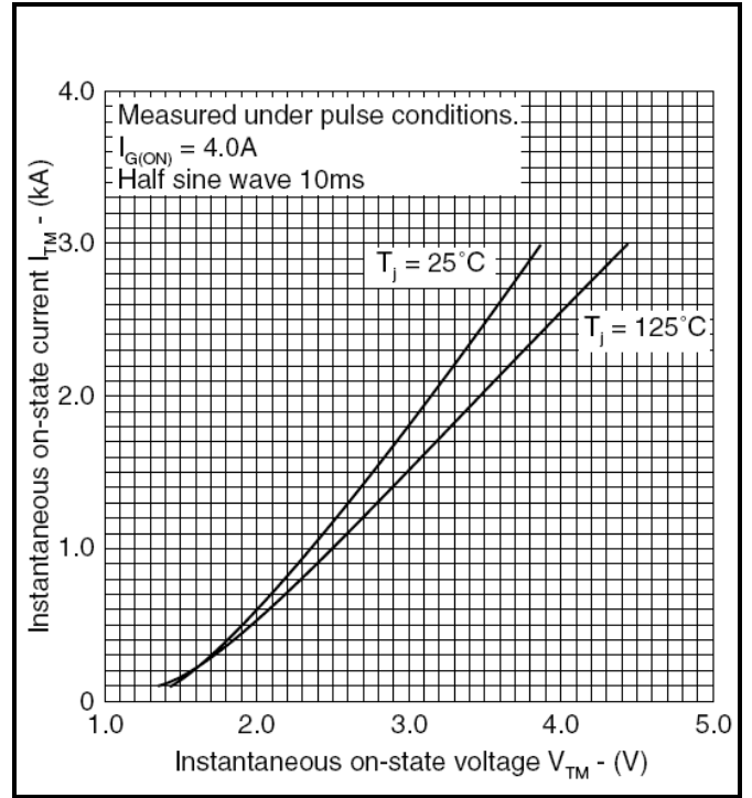
Fig.3 On-state characteristics
