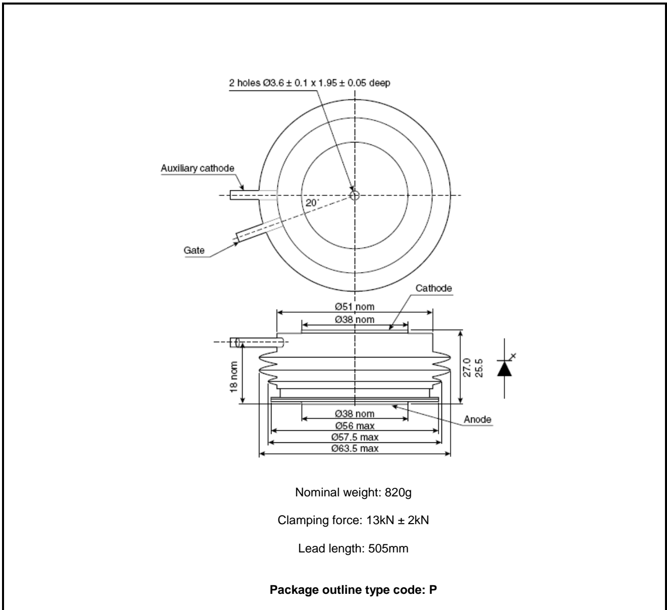
Fig. 31 Package outline
