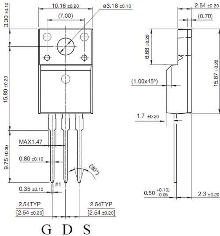
TO-220F
