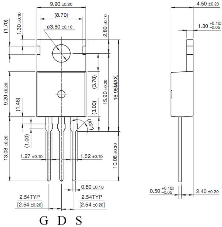
TO-220
