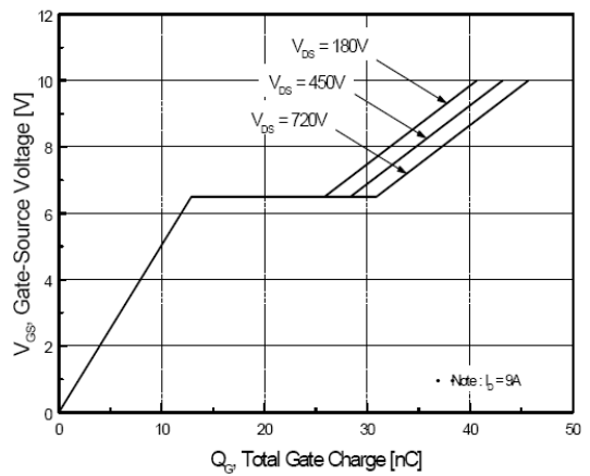
图6. 栅电荷特性曲线 Fig. 6 Gate Charge Characteristics
