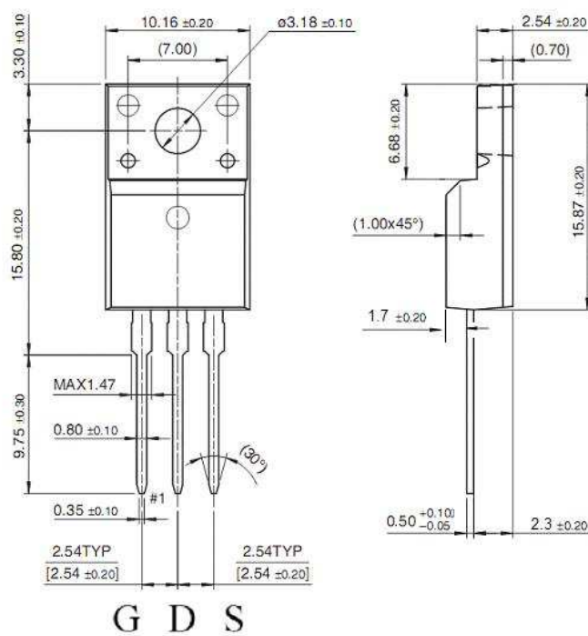
TO-220F
