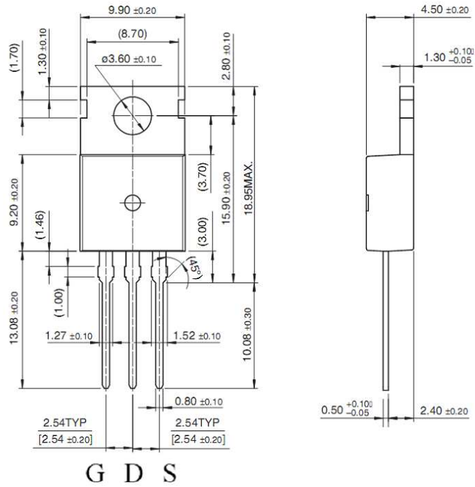
TO-220
