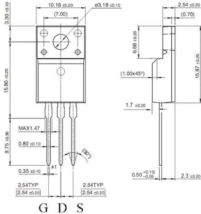
TO-220F
