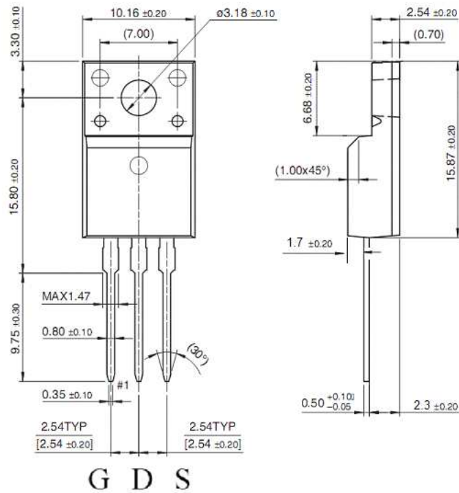
TO-220F
