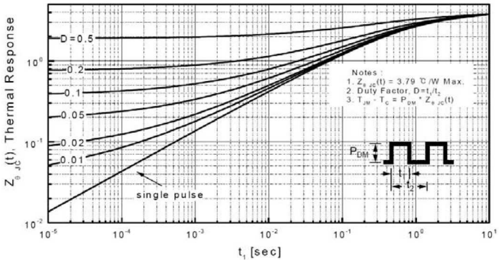
图10. 瞬态热响应曲线(TO-220F) Fig. 10 Transient Thermal Response Curve(TO-220F)
