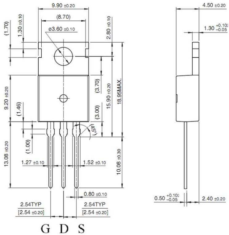
TO-220
