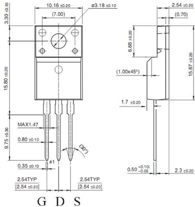
TO-220F
