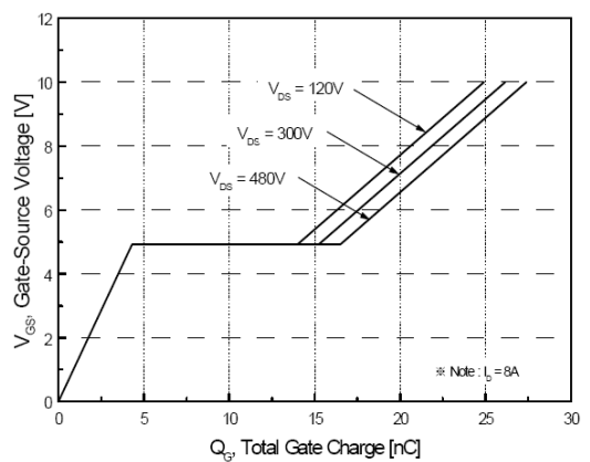
图6. 栅电荷特性曲线 Fig. 6 Gate Charge Characteristics
