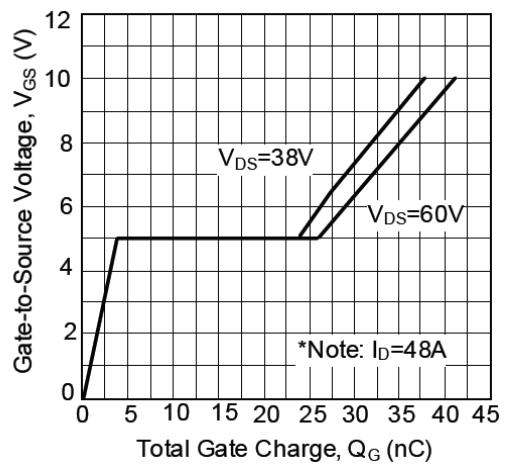
图6. 栅电荷特性曲线 Fig. 6 Gate Charge Characteristics
