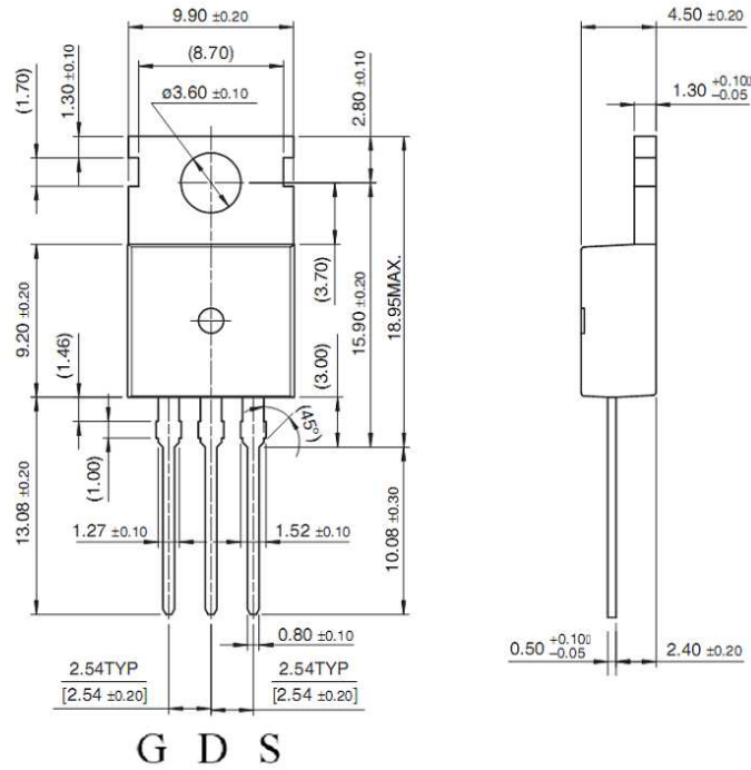
TO-220
