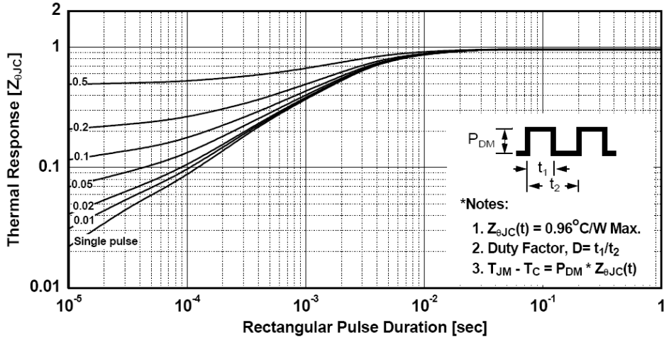
图9. 瞬态热响应曲线(TO-220) Fig. 9 Transient Thermal Response Curve (TO-220)
