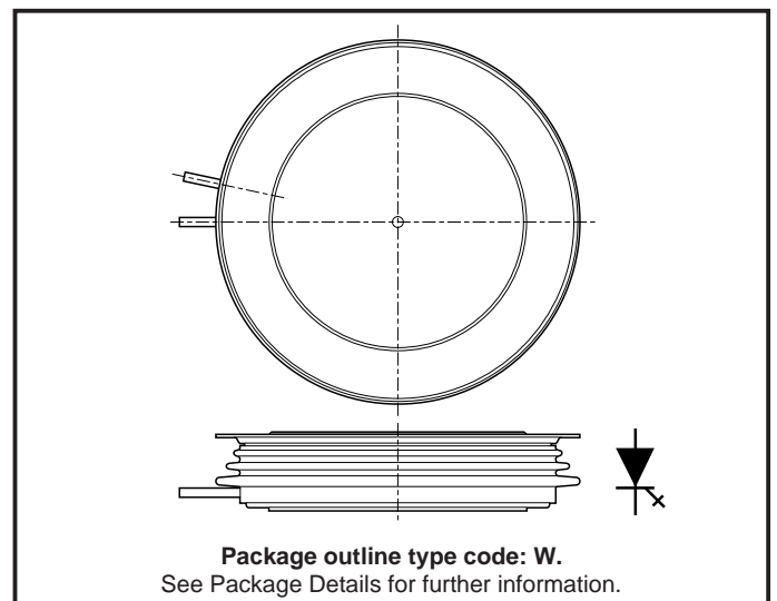
Figure 1. Package outline
