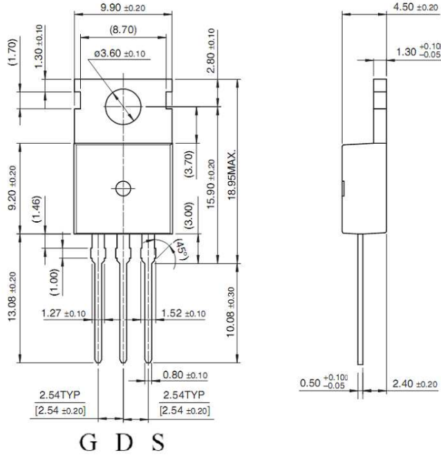
TO-220
