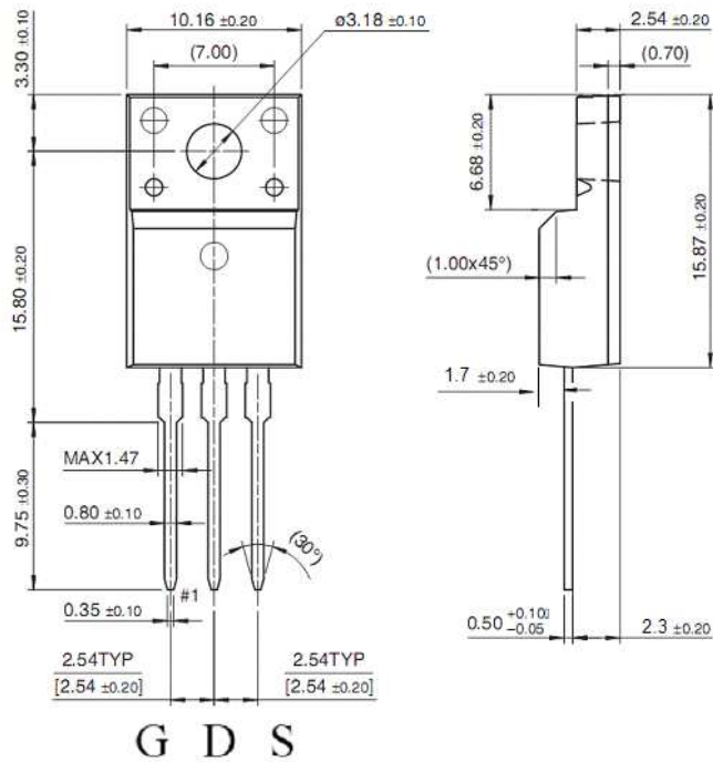
TO-220F
