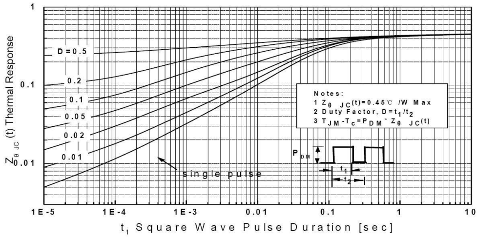
图9. 瞬态热响应曲线(TO-247) Fig. 9 Transient Thermal Response Curve(TO-247)
