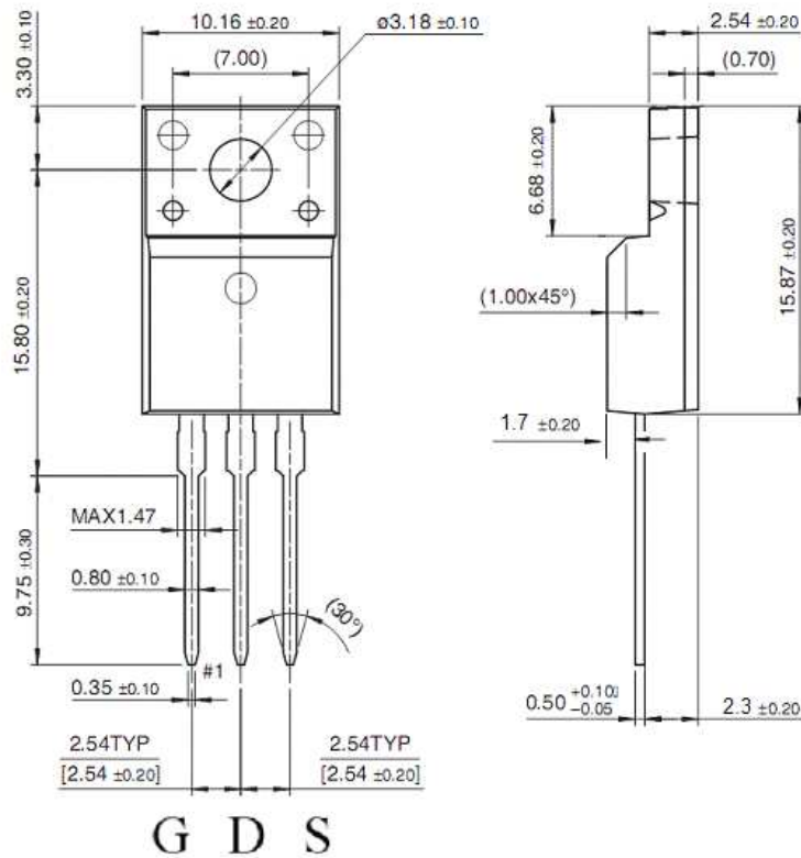
TO-220F
