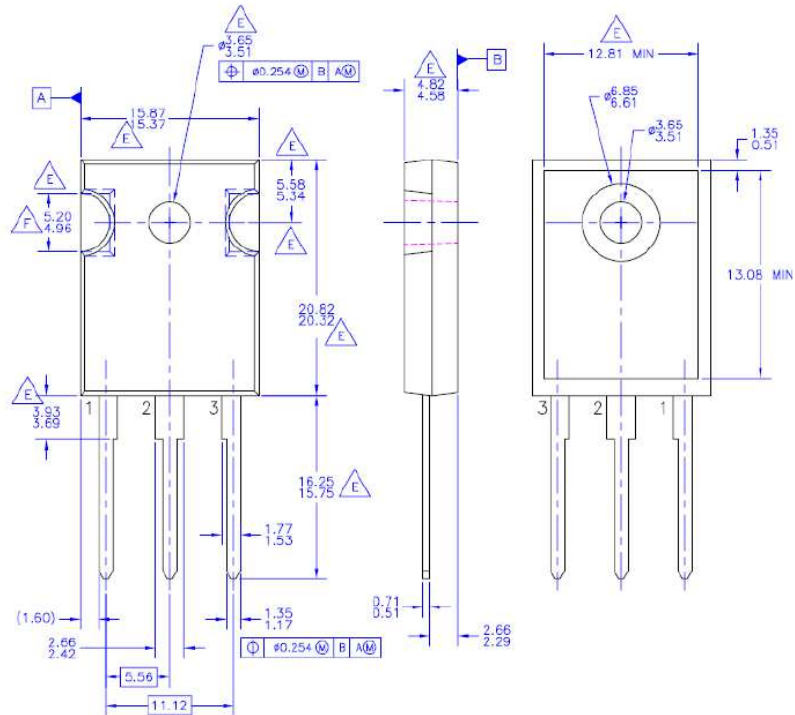
TO-247
