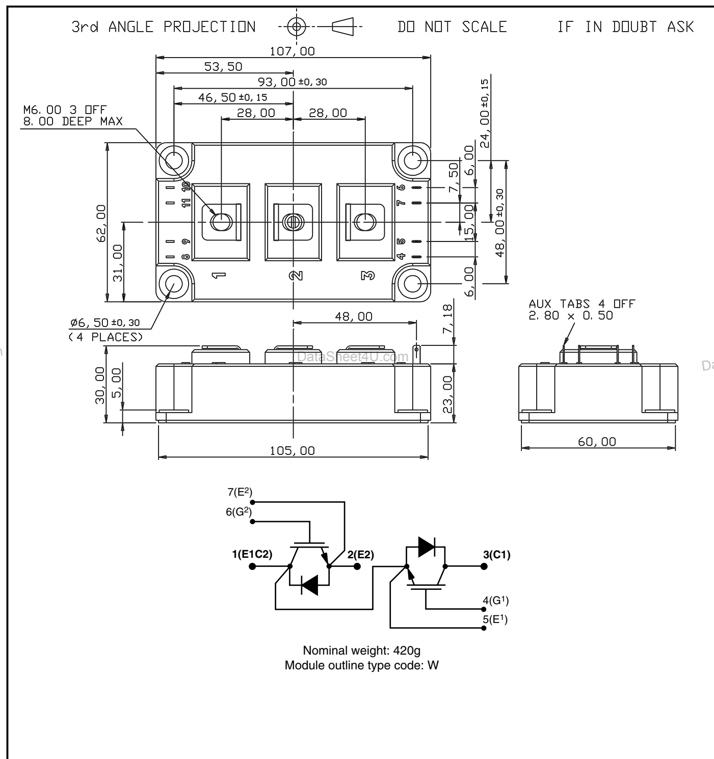
Fig. 11 Package details
