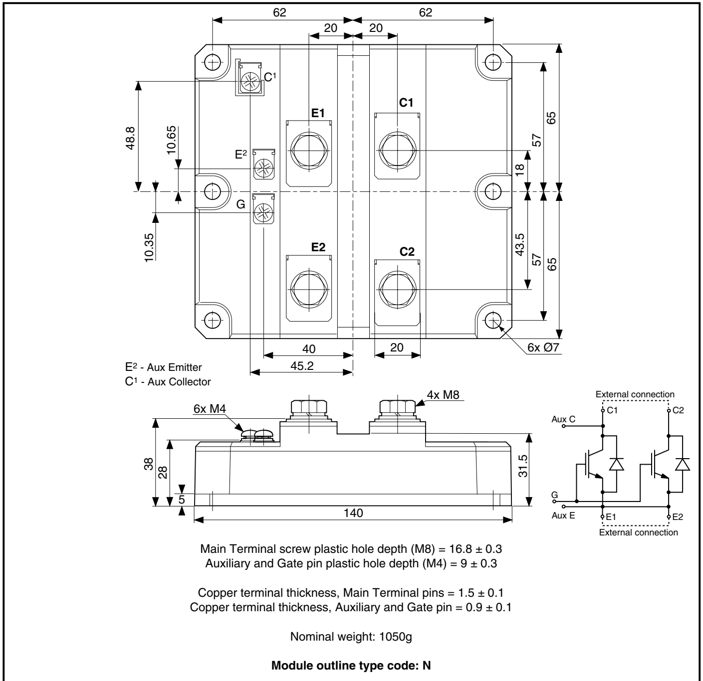
Fig. 11 Package details
