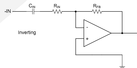
Figure 2 Inverting Gain Configuration
