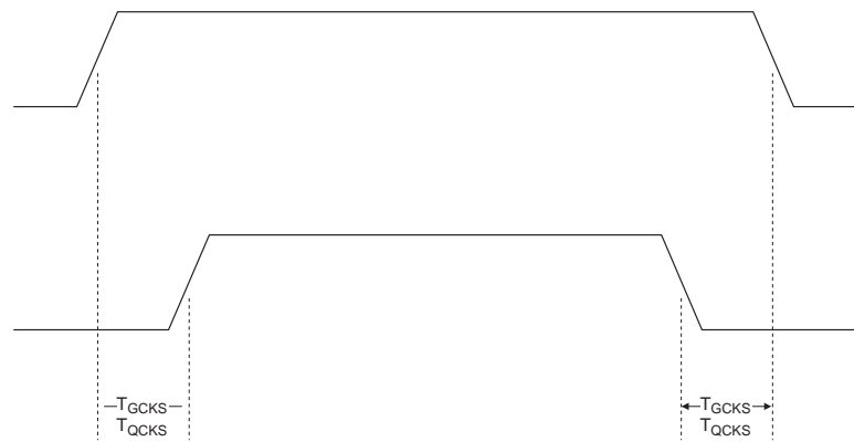
Figure 36: Global and Quadrant Clock Buffer Skew
