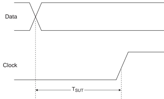
Figure 21: Logic Block T-Flip Flop Setup Time
