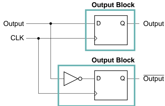
Figure 9: Differential outputs
