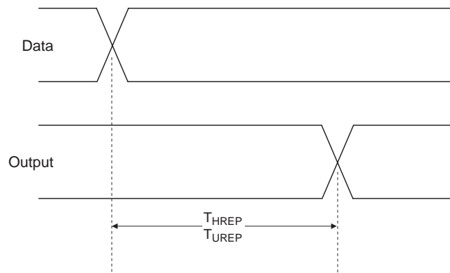
Figure 16: Repeater Delays
