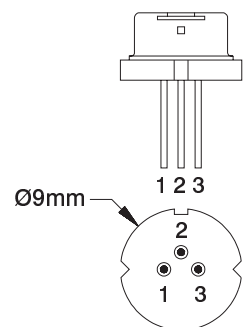
Package Type: Ø9mm
