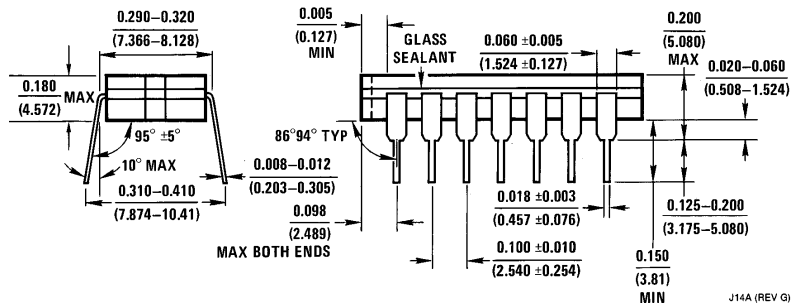
14-Lead Ceramic Dual-In-Line Package (J) Order Number DM5405J NS Package Number J14A
