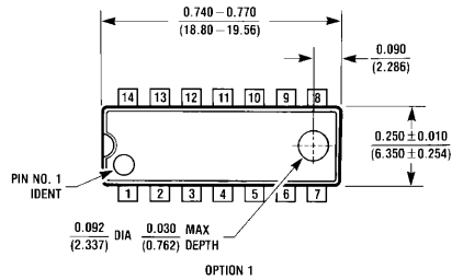
14-Lead Ceramic Dual-In-Line Package (J) Order Number DM5405J NS Package Number J14A
