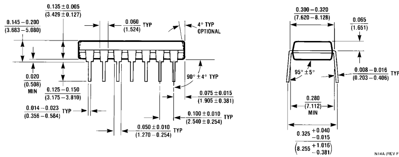
14-Lead Molded Dual-In-Line Package (N) Order Number DM7405N NS Package Number N14A
