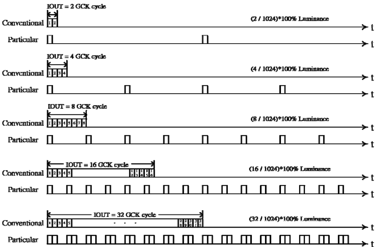
Figure 7. The Progressive PWM Method (1)
