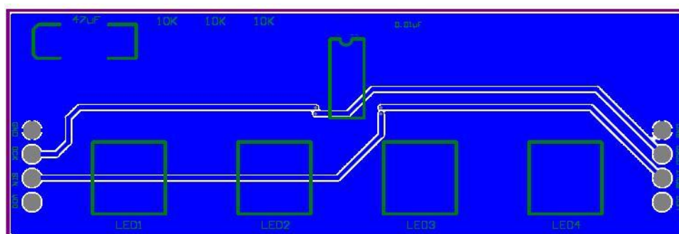
Bottom View
