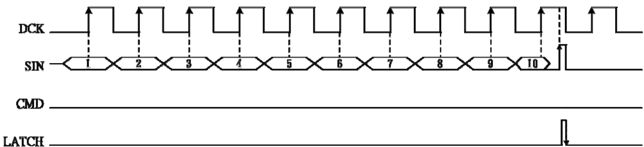
Figure 11. The timing diagram of grayscale data
