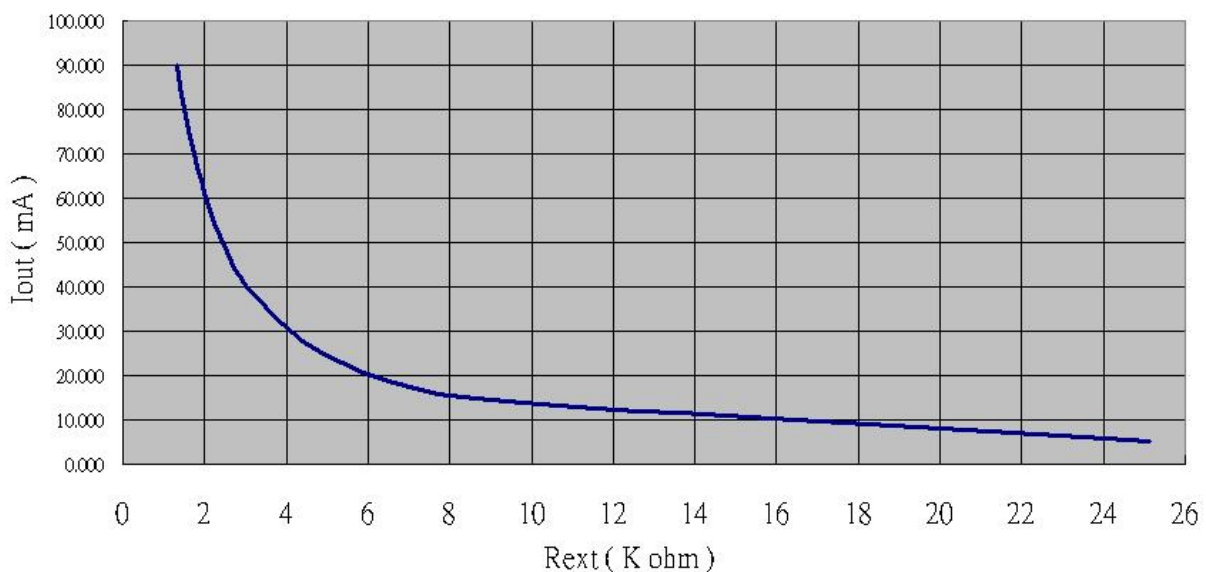
Figure 15. IOUT V.S. Rext curve
