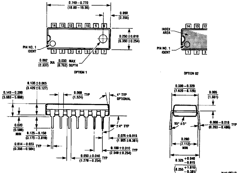
Molded Dual-In-Line Package (N) Order Number DM74AS1036AN NS Package Number N14A
