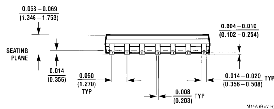
14-Lead Small Outline Molded Package (M) Order Number DM74LS393M NS Package Number M14A
