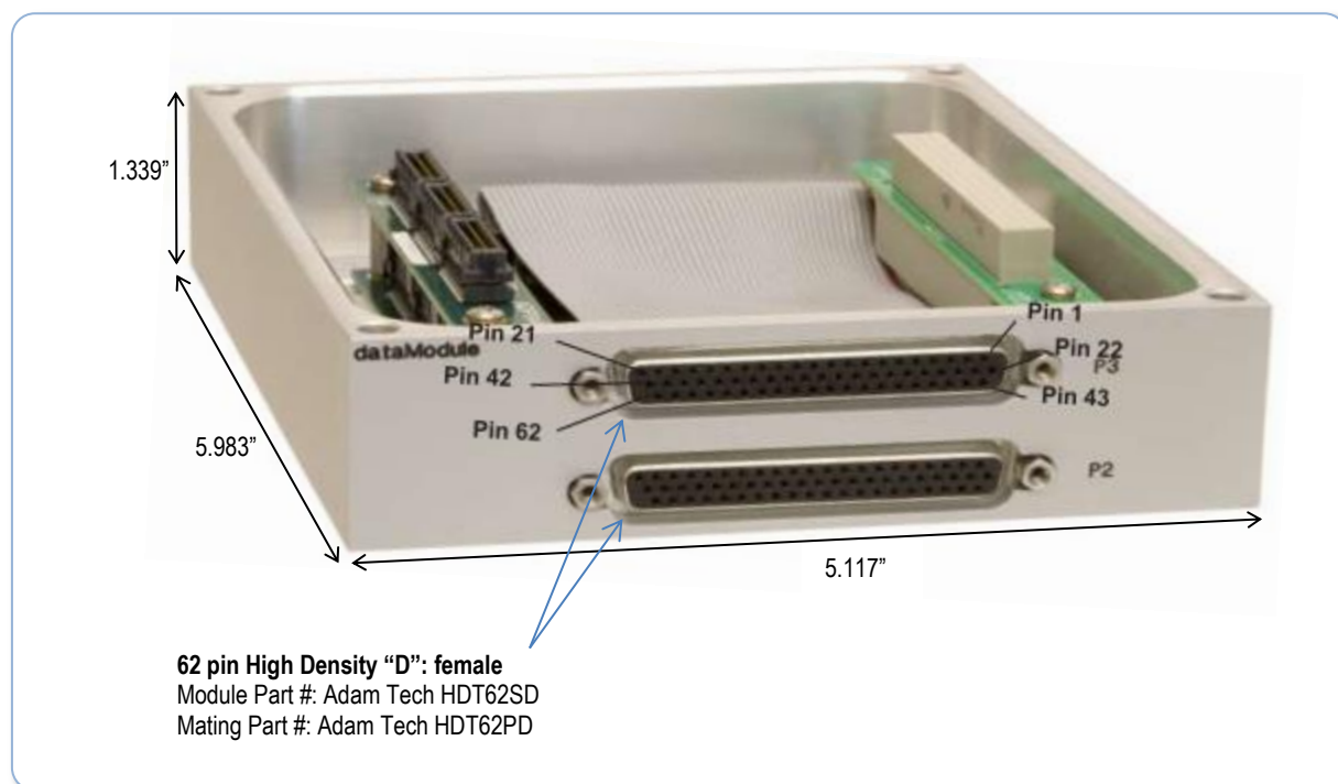
Figure 4: IDAN Dimensions
