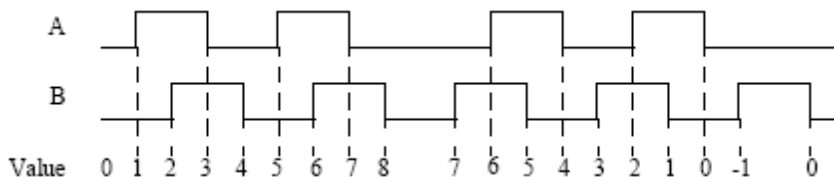
Figure 11: Incremental Encoder Signals
