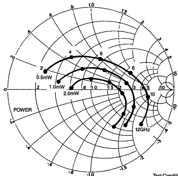
Test Conditions R_L = 10 \text{ ohms}
