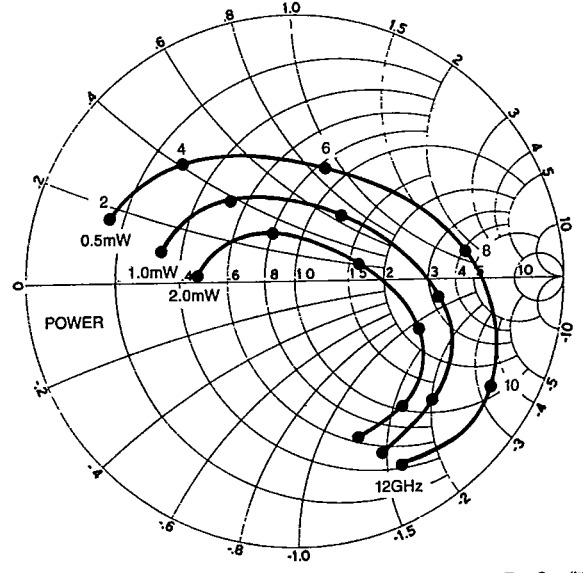
Test Conditions R_L = 10 ohms
