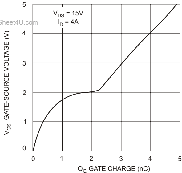
Fig. 7 Gate-Charge Characteristics
