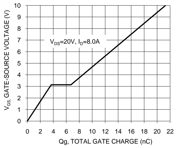
Figure 12. Gate Charge
