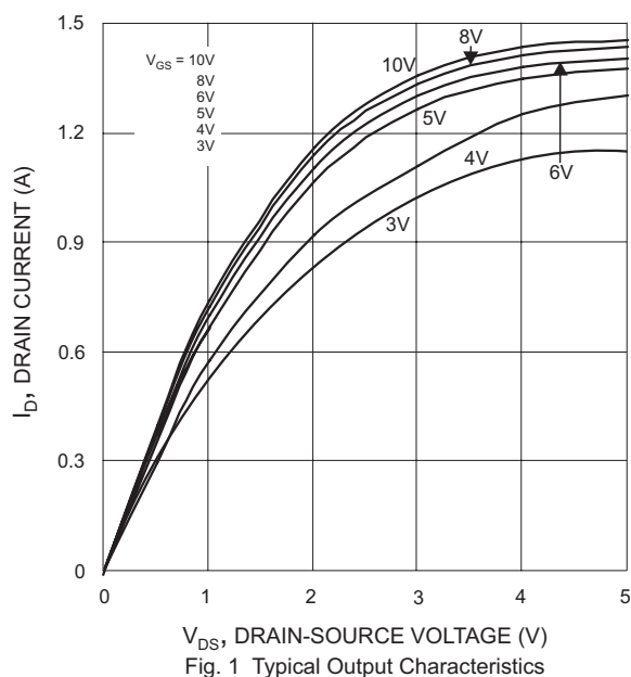
Fig. 1 Typical Output Characteristics
