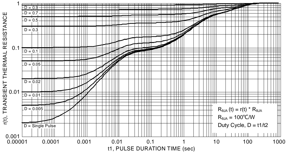
Figure 12 Transient Thermal Resistance
