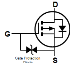
Equivalent Circuit
