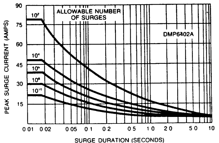
Figure 2. Peak Surge Current vs Duration, AC Output Module
