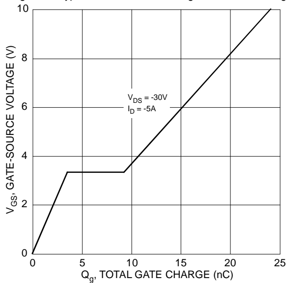
Figure 12 Gate-Charge Characteristics
