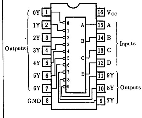
ピン配置図(上面図)/Pin Assignment
