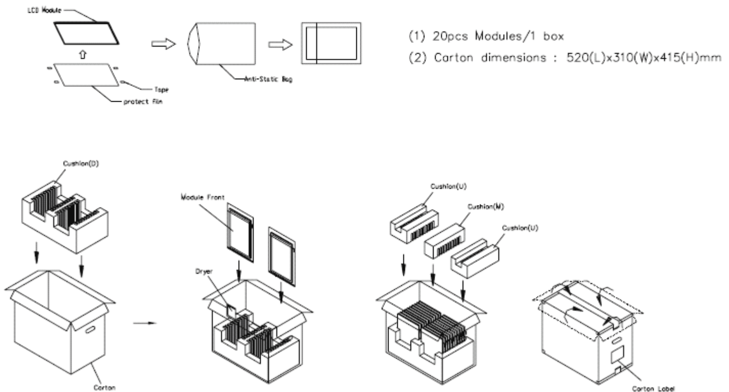
Figure. 9-1 Packing method
