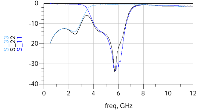
Return Loss
