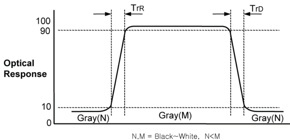
FIG. 11 Response Time
