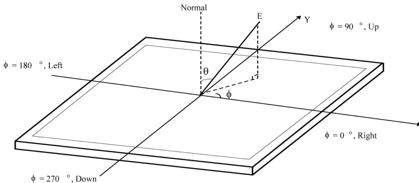
FIG.12 Viewing Angle
