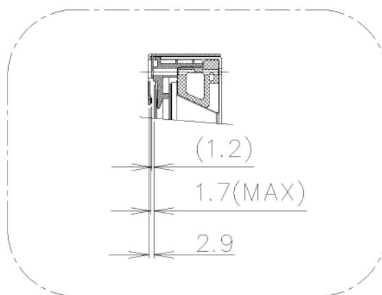
SEC. A~A' SCALE=1/4
