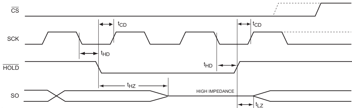
Figure 2. HOLD Timing
