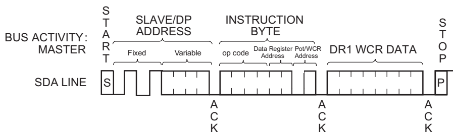
Figure 6. Write Timing
