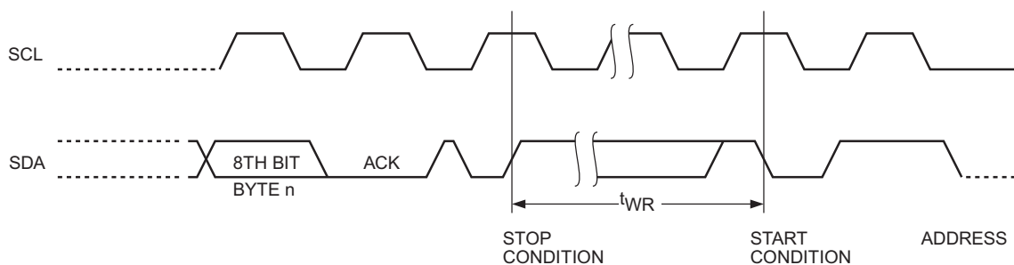
Figure 3. Start/Stop Timing
