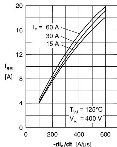
Fig. 3 Typ. reverse recovery current I_{RM} versus -di_F/dt
