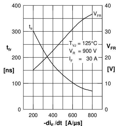
Fig. 6 Typ. forward recov. voltage V_{FR} & time t_{fr} versus di_F/dt
