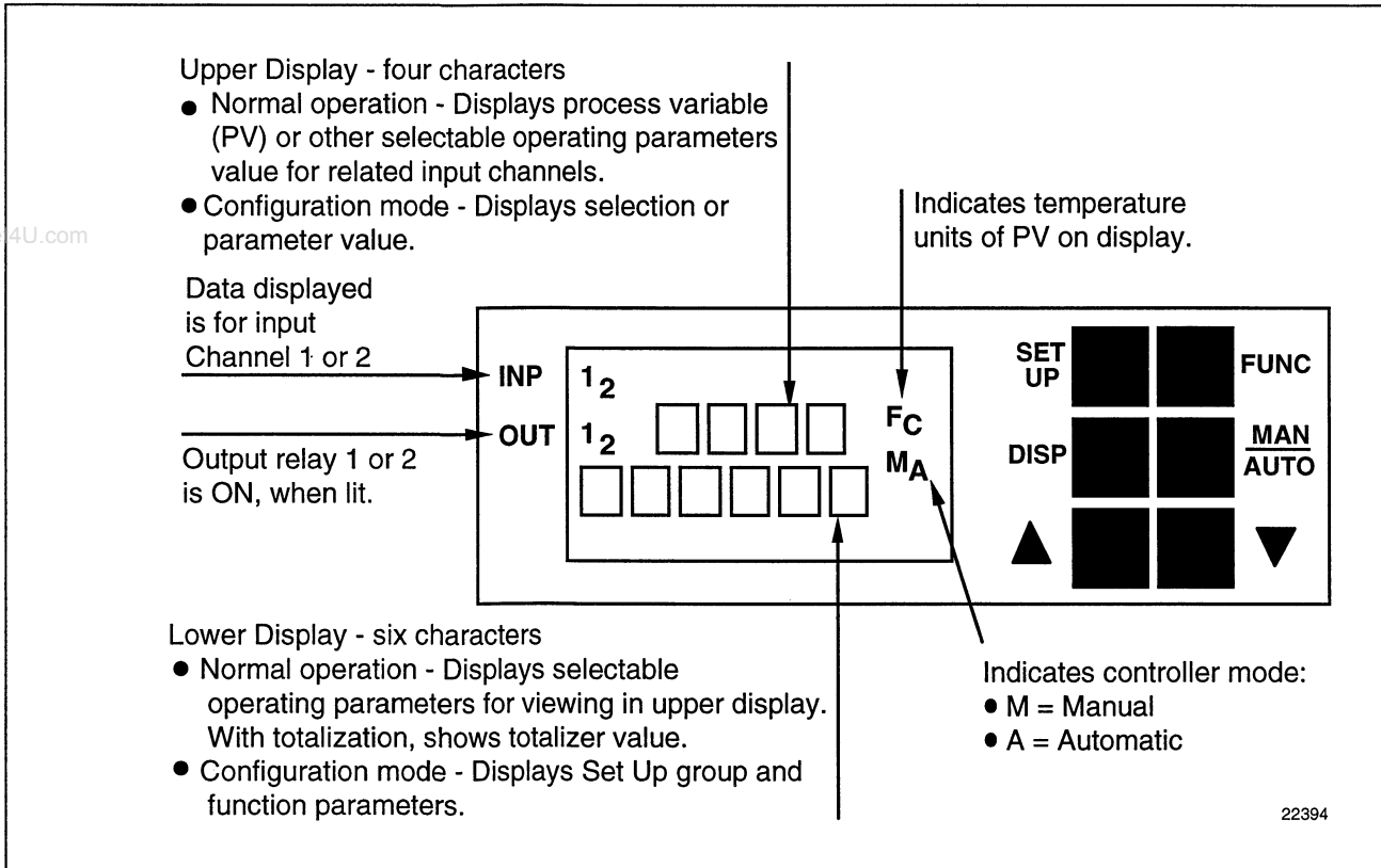
Figure 1-4 Operator Interface
