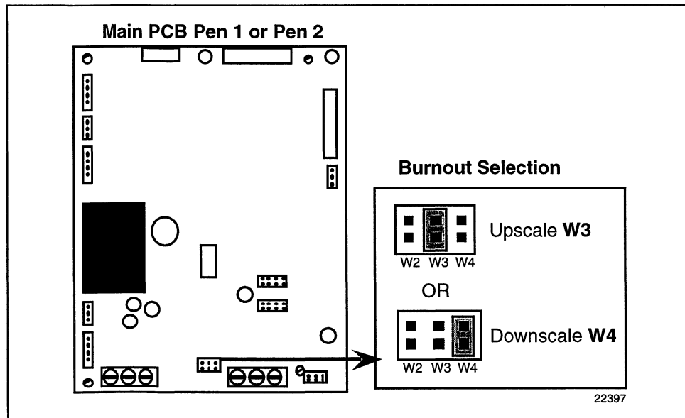
Figure 2-3 Jumpers W3/W4 Positions (Burnout)
