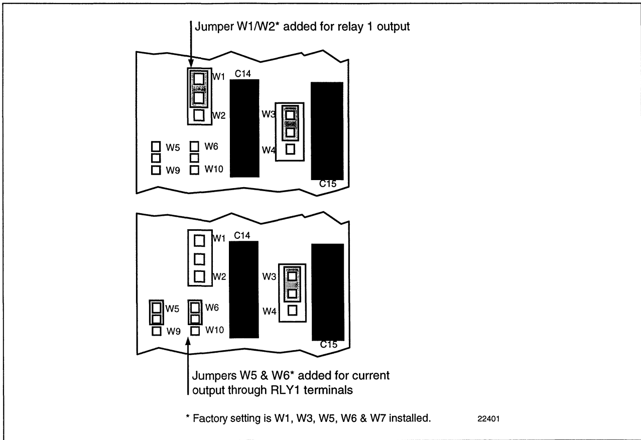
Figure 2-7 Jumper Positions for Relay and Current Output on Control PCB 30756087-001
