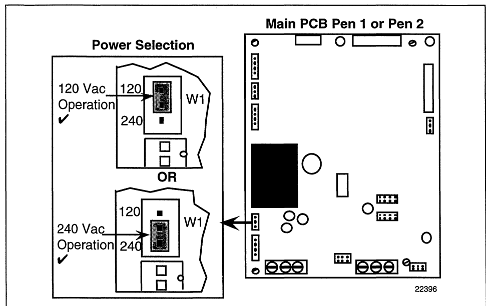
Figure 2-2 Jumper W1 Positions (AC Line Power)
