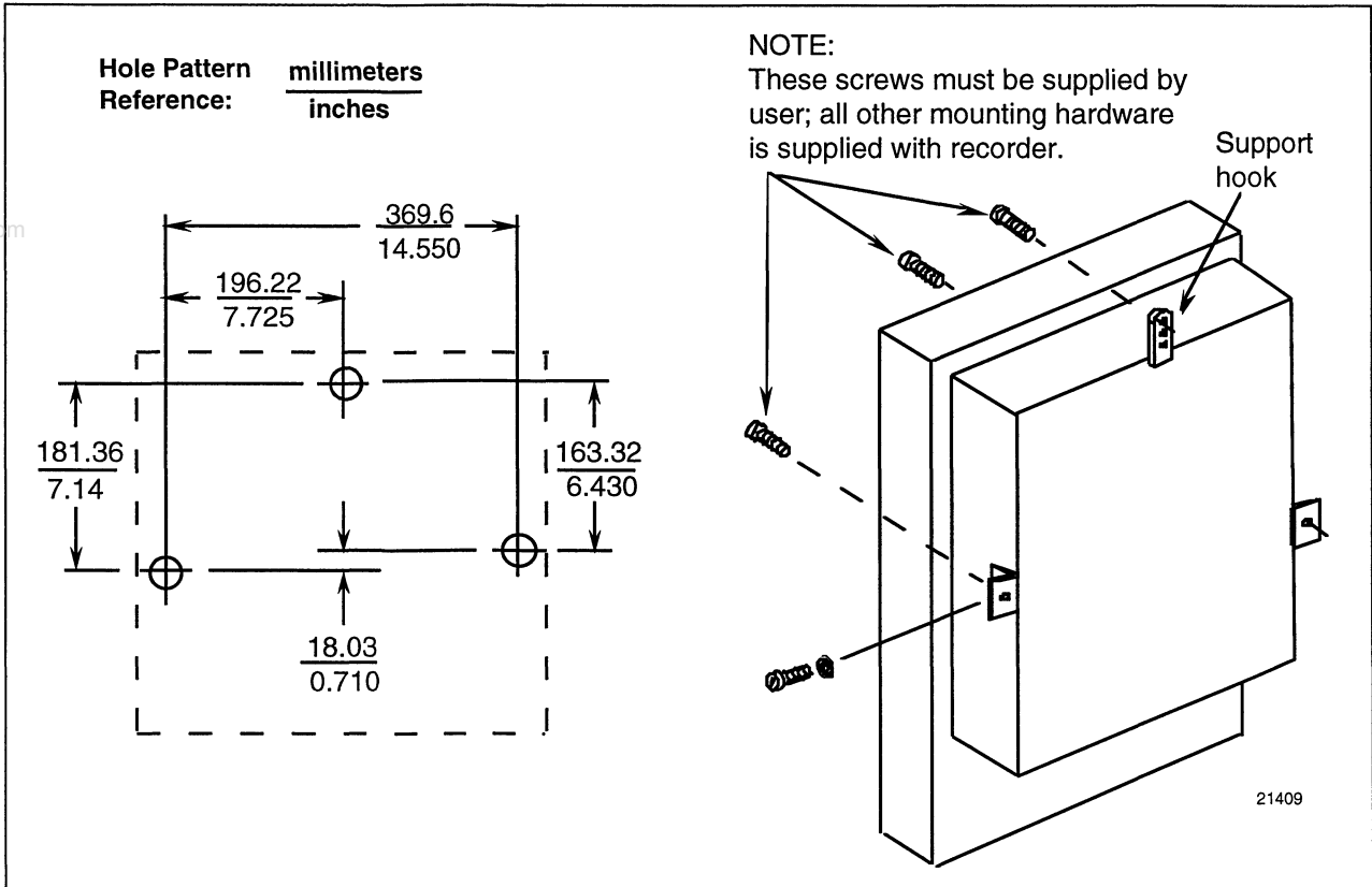
Figure 3-4 Mounting Flush on a Surface (of Panel or Wall)
