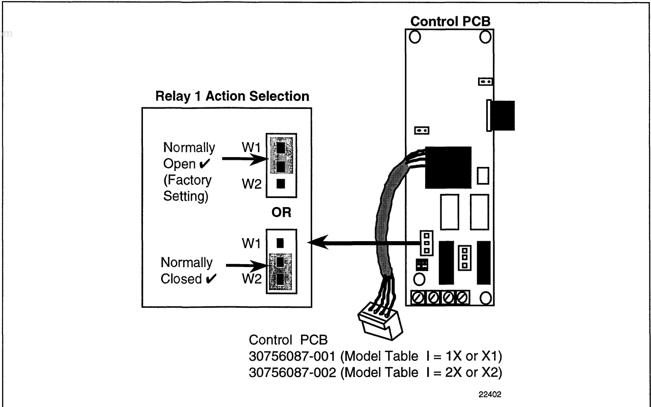
Figure 2-8 Jumper Locations for Relay #1 Action
