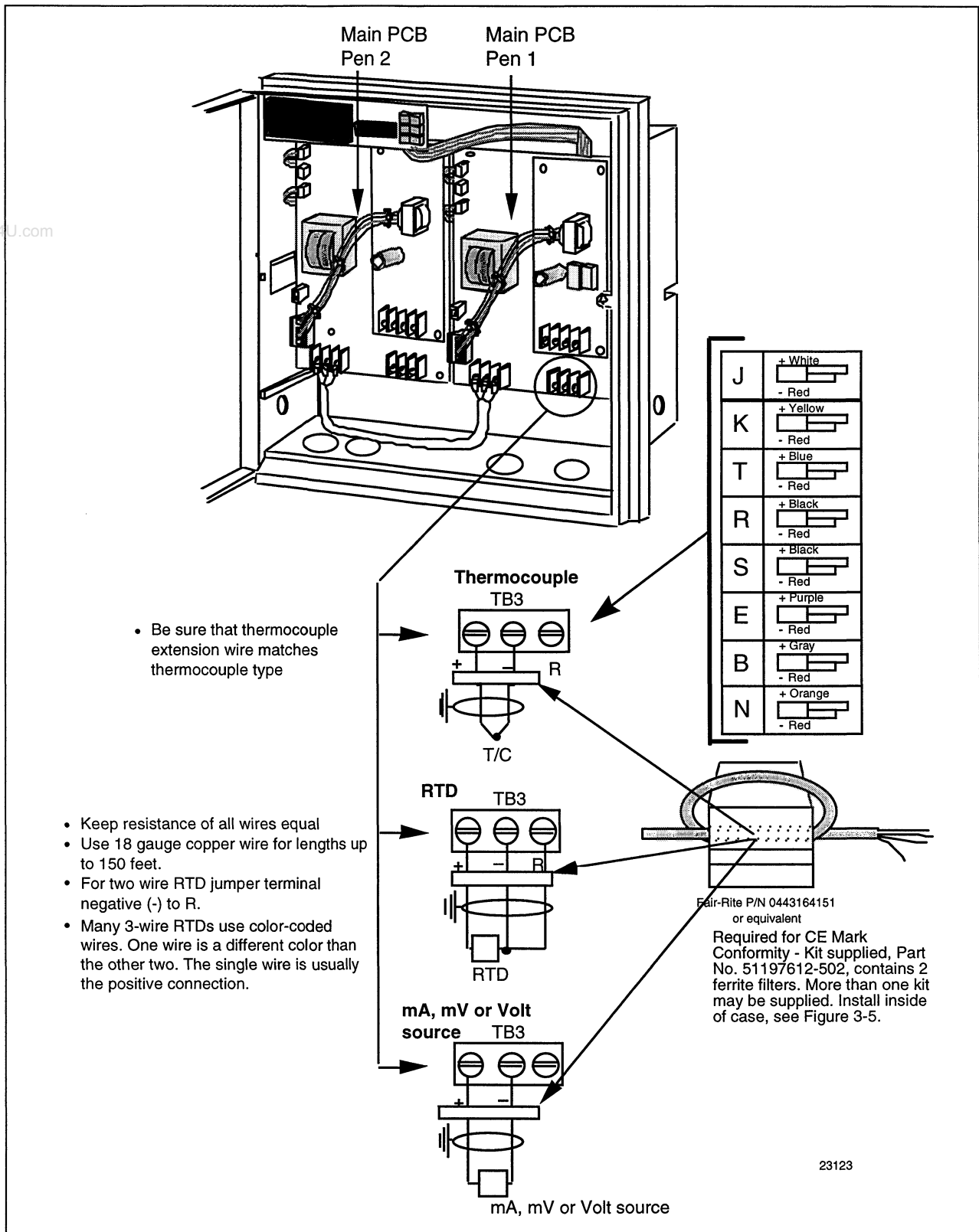
Figure 3-7 Input 1 Wiring
