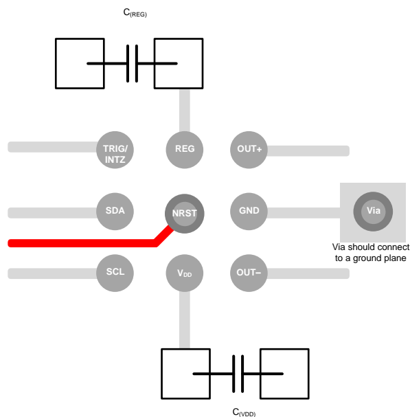
Figure 97. Typical Layout
