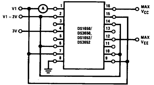
FIGURE 5. I_{IH}
