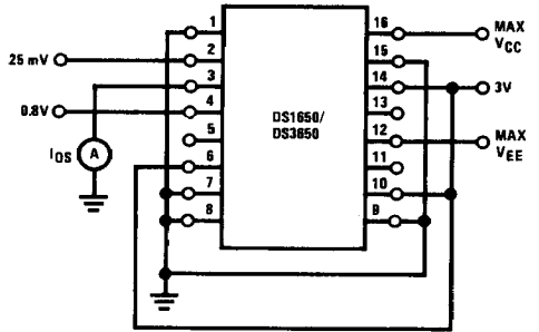
FIGURE 4. I_{OS}
