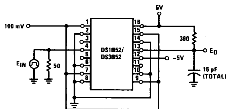
FIGURE 10. Strobe Propagation Delay t_{PLH}(S) and t_{PHL}(S)
