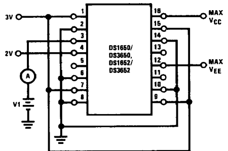
FIGURE 5. I_{IH}
