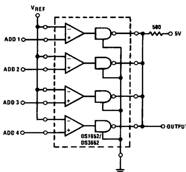
Implied "AND" Gating
