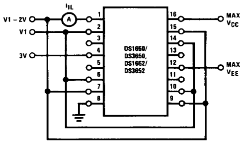
FIGURE 6. I_{IL}
