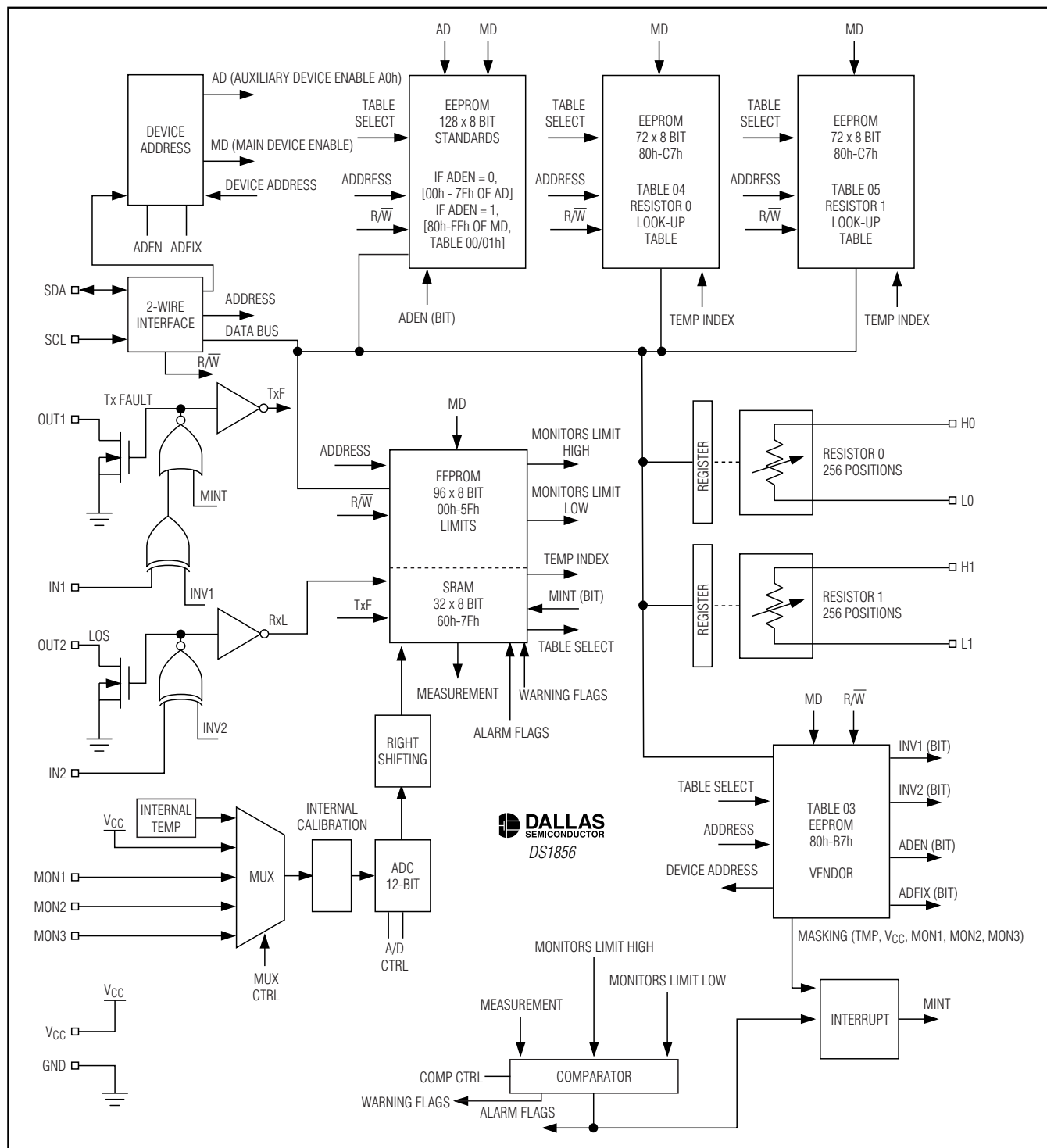
Figure 1. Block Diagram
