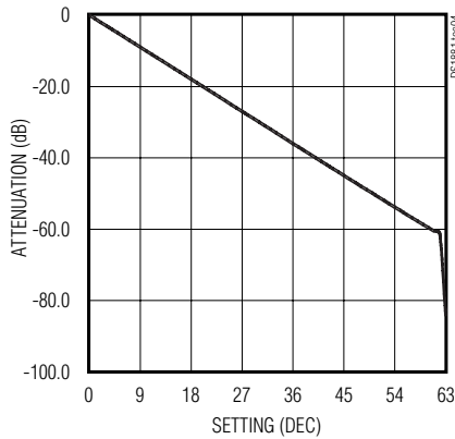
POTENTIOMETER 1 (CONFIGURATION 2) ATTENUATION vs. SETTING
