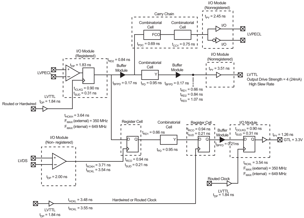
Figure 20 • Timing Model
