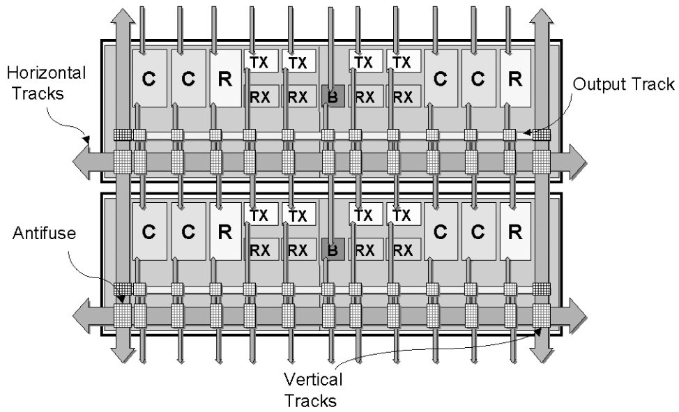
Figure 61 • Horizontal and Vertical Tracks
