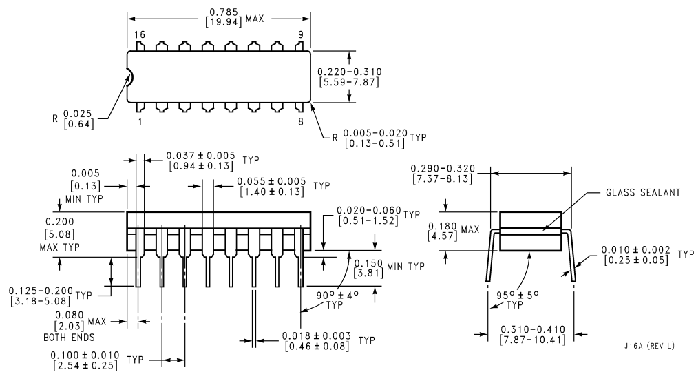
Ceramic Dual-In-Line Package (J) Order Number DS26F32MJ/883 NS Package Number J16A
