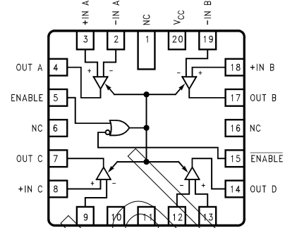
20-Lead Ceramic Leadless Chip Carrier
