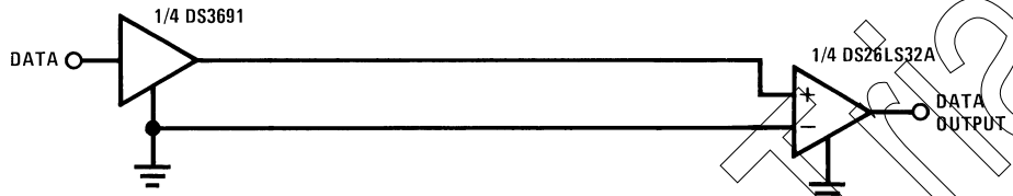
Single Wire with Driver Ground Reference—RS-423
